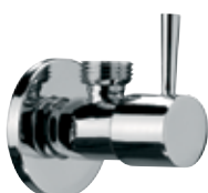
128L1238 € 14,00 Rubinetto sottolavabo "MINIMAL", con vitone ceramico, con maniglia a leva, 1/2x3/8. C.P. brass "MINIMAL" angle valve, with ceramic head valve, with lever handle, 1/2x3/8.
