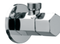
128E1238 € 18,90 Rubinetto sottolavabo "Esagonale", con vitone ceramico, 1/2x3/8. C.P. brass "Hexagonal" angle valve, with ceramic head valve, 1/2x3/8.
