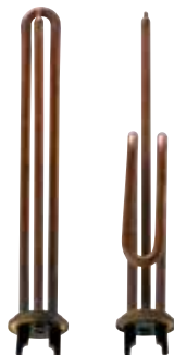
1121 €11,50 Resistenza per scaldabagno attacco con flangia, Watts 1200. Straight heating element for water heater, 1"1/4, flanged cap, Watts 1200.
