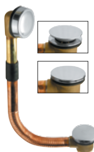
96CC € 56,20 Colonna di scarico con tubo in rame, con pileta "click-clack". C.P. brass waste and overflow with copper tube and "click-clack" waste.
